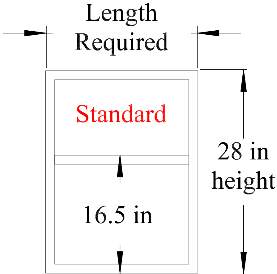
1.25" x 1.25" square aluminum tubing
